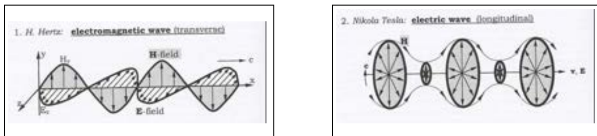
Fig. 1: A transversal electromagnetic wave and a longitudinal scalar wave. Meyl (2003)
